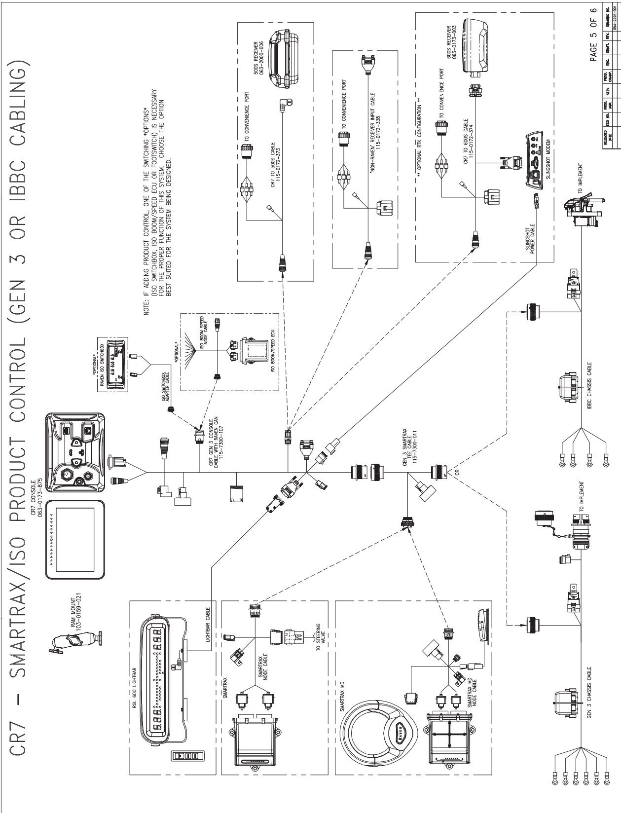
FIGURE 6. Gen 3 or IBBC Cabling CR7 SmarTrax ISO Product Control
