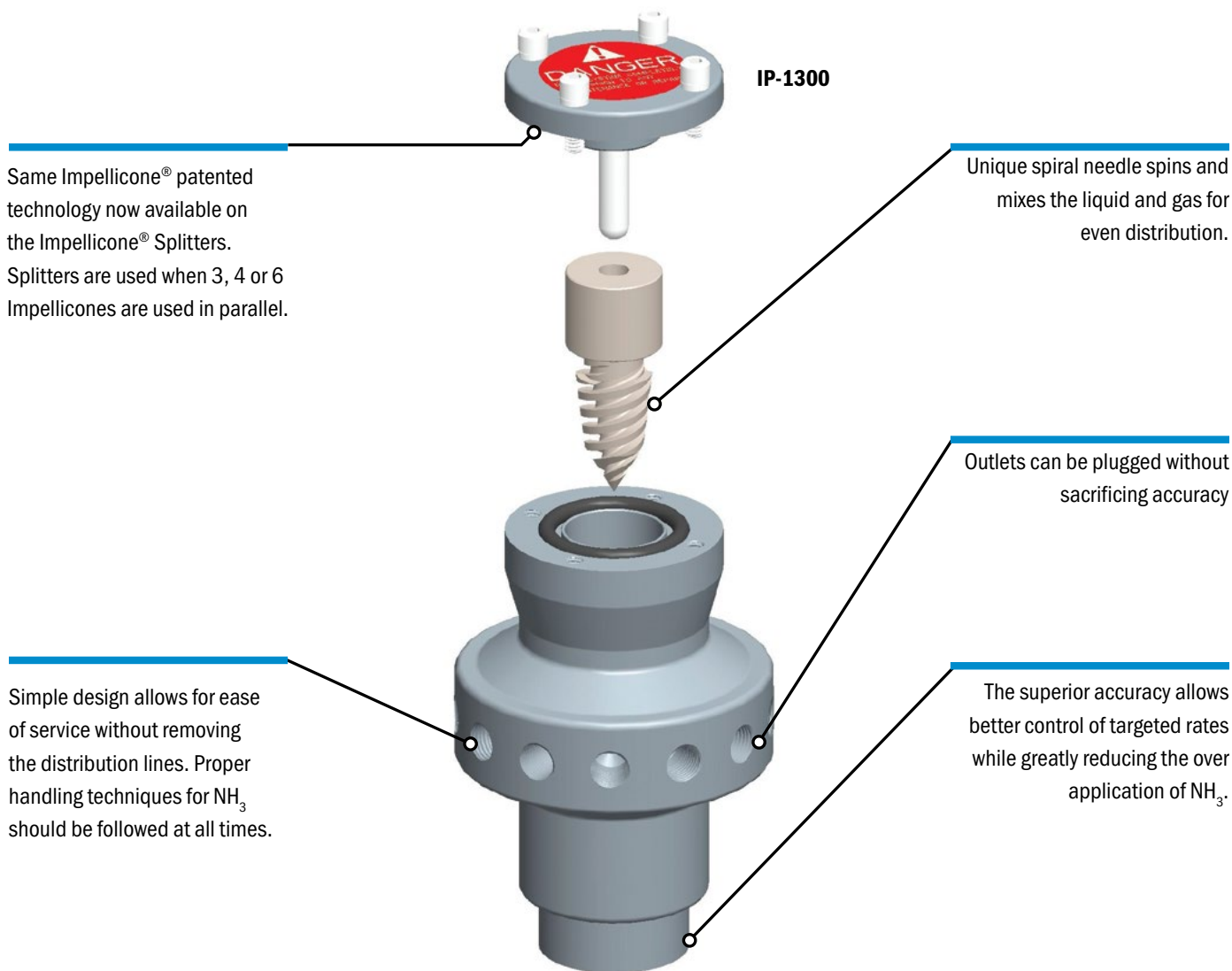
Impellicone® Flow Dividers, Splitters, and Manifolds
